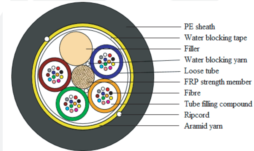
ADSS-SS-200m-48B1.3 Schematic for reference only
