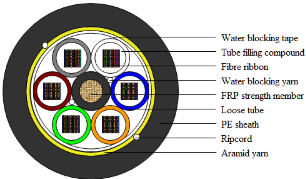
ADSS-SS-150m-864B1.3-12F Structure of other fibre counts refer to 3.4 Schematic for reference only
